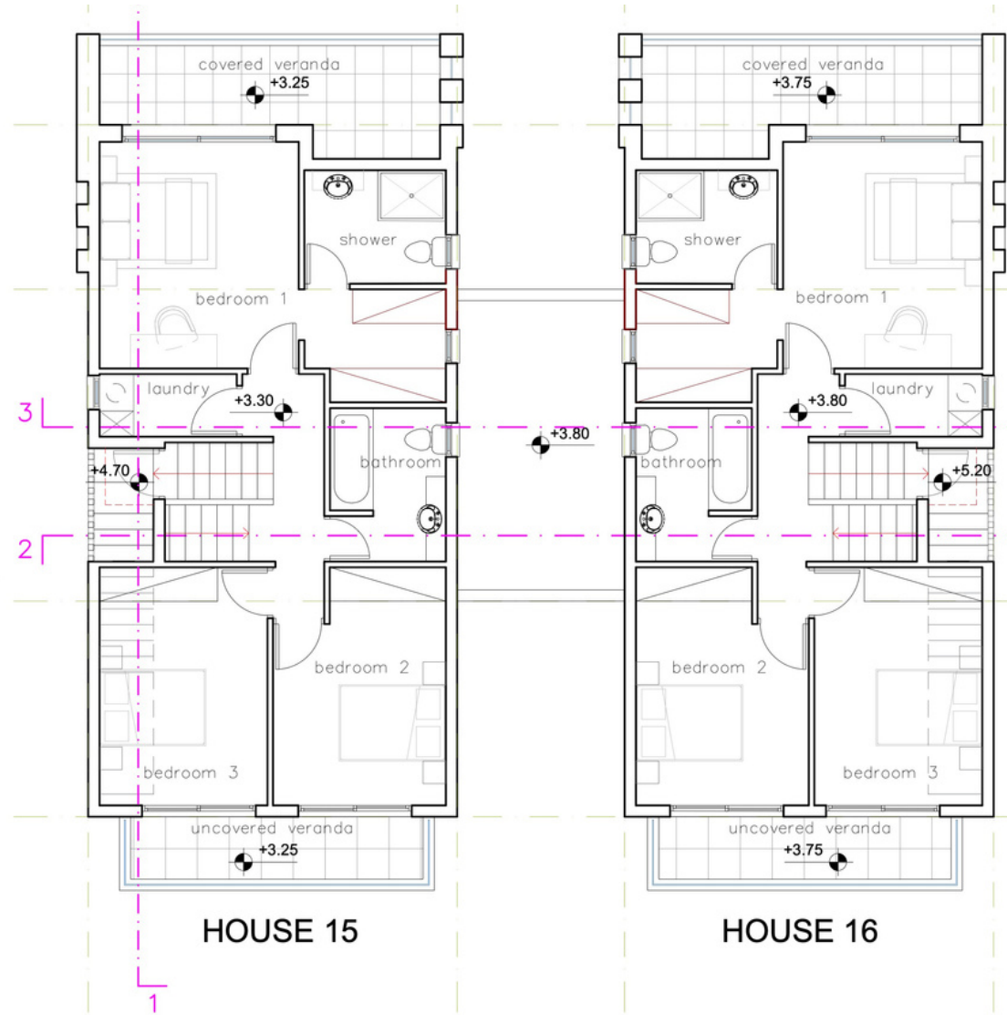
FIRST FLOOR
