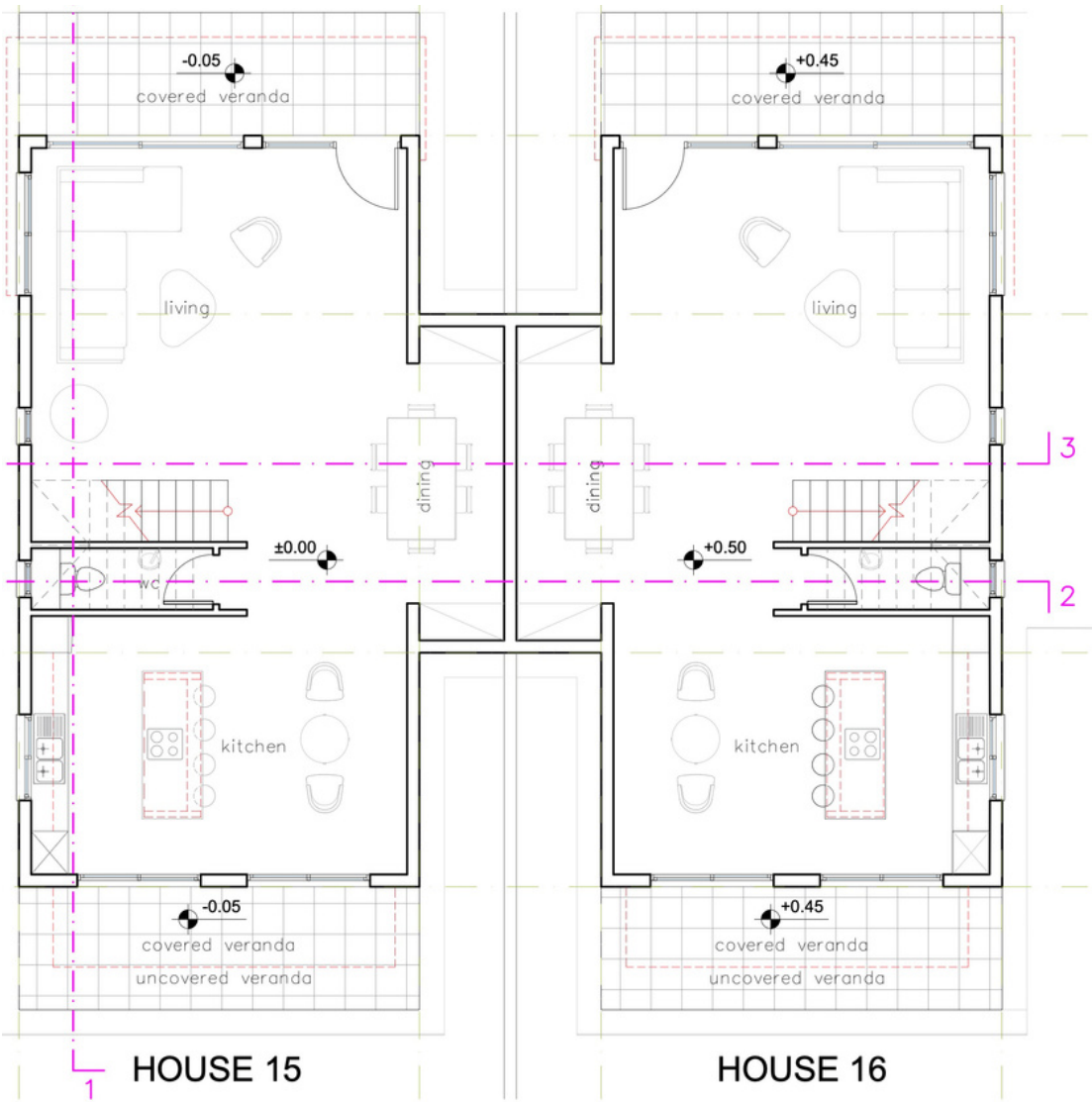
GROUND FLOOR
